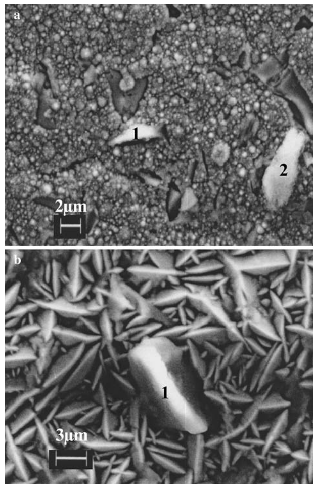
Fig. 9 Surface morphology of corroded Ni-38Co-YZA (a) and Ni-85Co-YZA (b) composites revealing the \text{Al}_2\text{O}_3 rich particle
