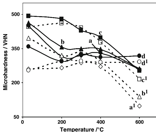
Fig. 10 Effect of heat treatment on microhardness of the coatings: Ni (a 1 ), Ni–YZA (a), Ni–17Co (b 1 ), Ni–17Co–YZA (b), Ni–38Co (c 1 ), Ni–38Co–YZA (c), Ni–85Co (d 1 ), Ni–85Co–YZA (d)
