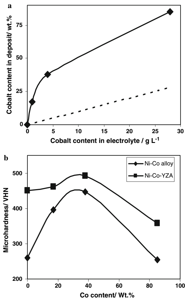
Fig. 5 Ni–Co anomalous codeposition (a) and the effect of Co content on the microhardness of Ni–Co alloys/Ni–Co–YZA composites (b)
